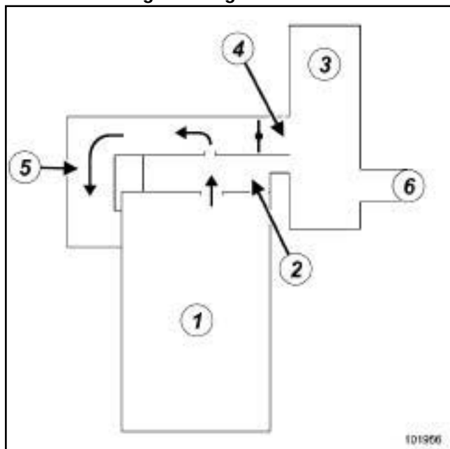
Operating diagram of the oil vapour rebreathing circuit for average and high loads
