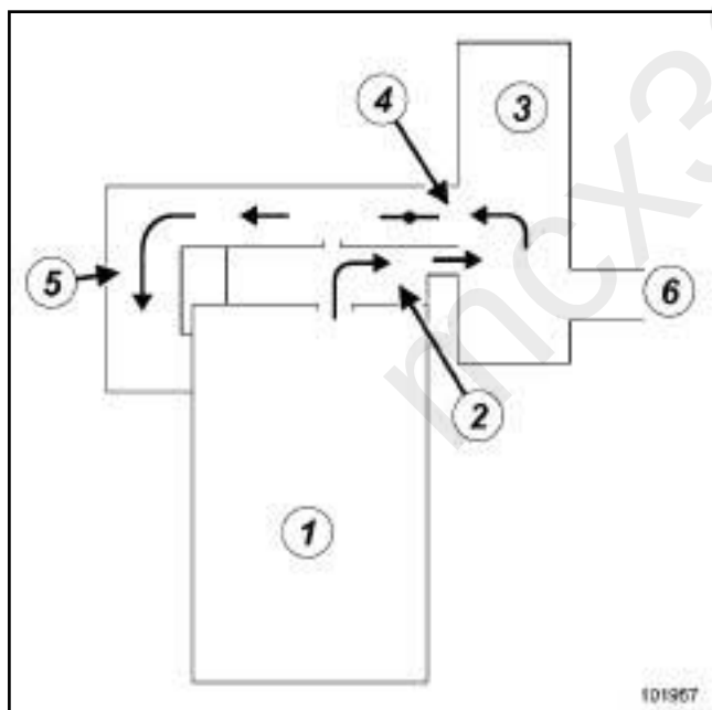
Operating diagram of the oil vapour rebreathing circuit for low loads
